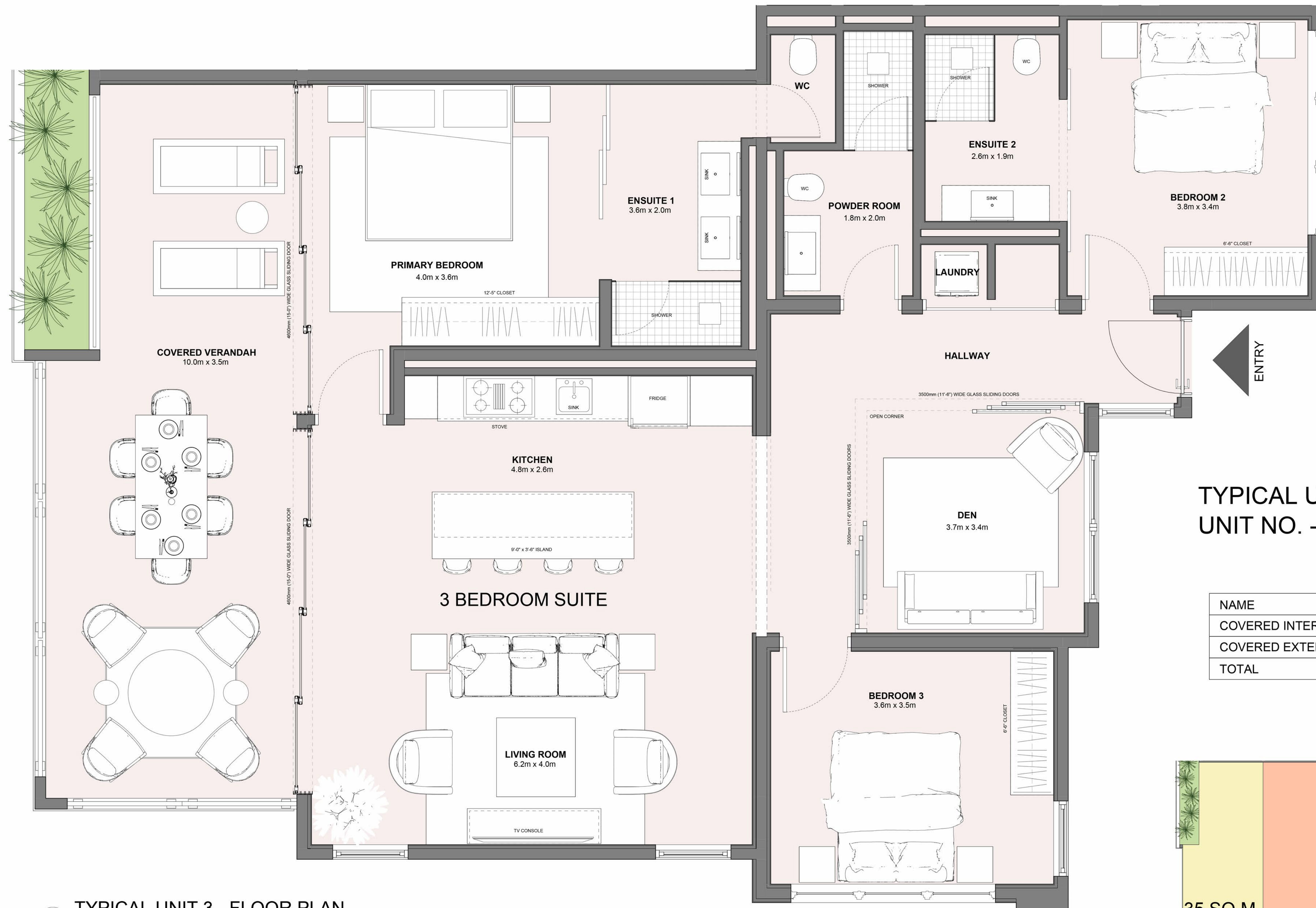
1 TYPICAL UNIT 3 - FLOOR PLAN 1 : 30
